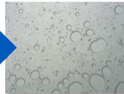
100x 1% Cetareth-20/ Cetearyl Alcohol
