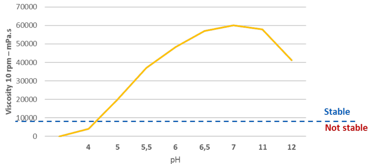
pH Tolerance: Emulsion 20% Almond Oil
