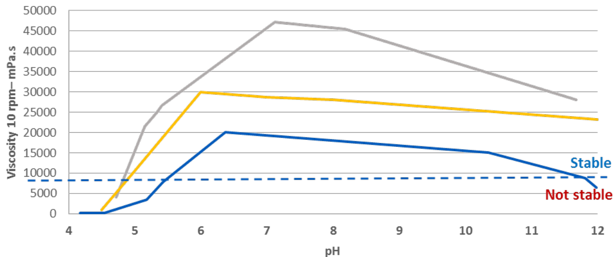
pH Tolerance: Water gel
