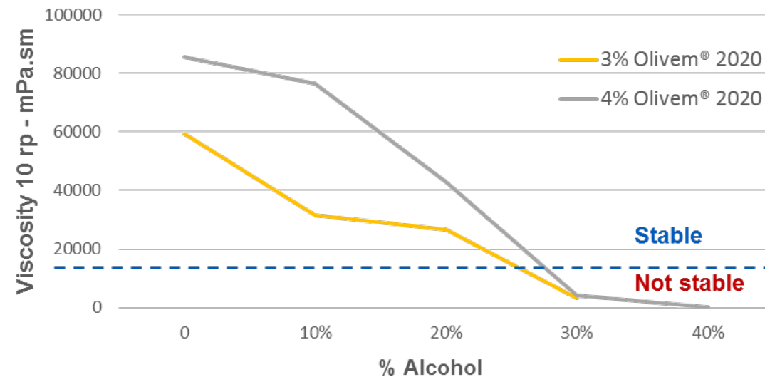
Alcohol Tolerance: Emulsions
